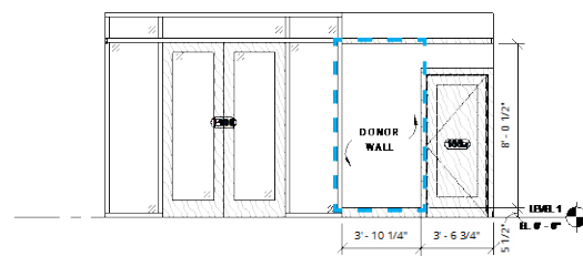
VESTIBULE - WEST ELEVATION
