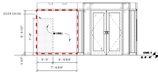
VESTIBULE - EAST ELEVATION
